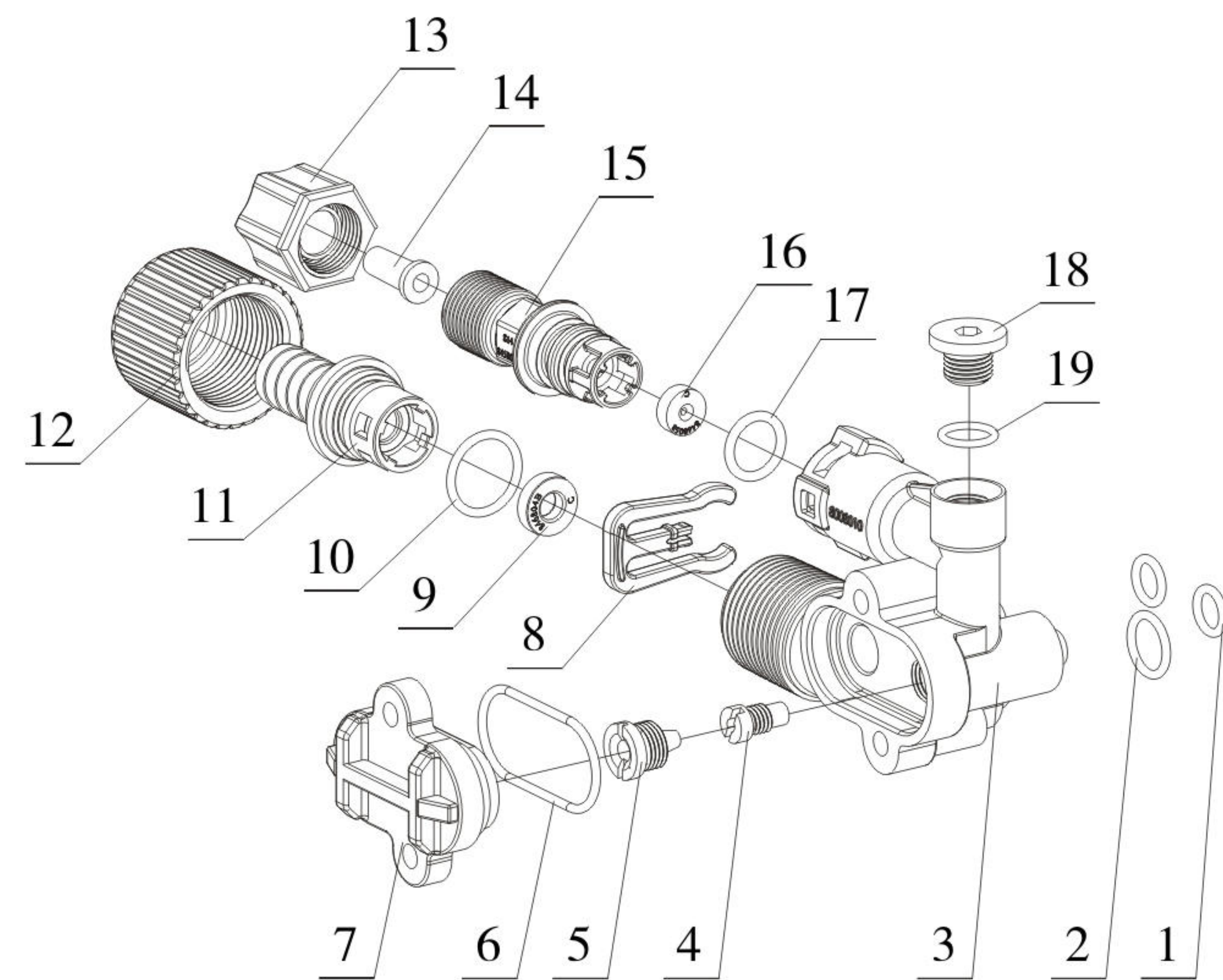
New Injector (6800 series) Components:
