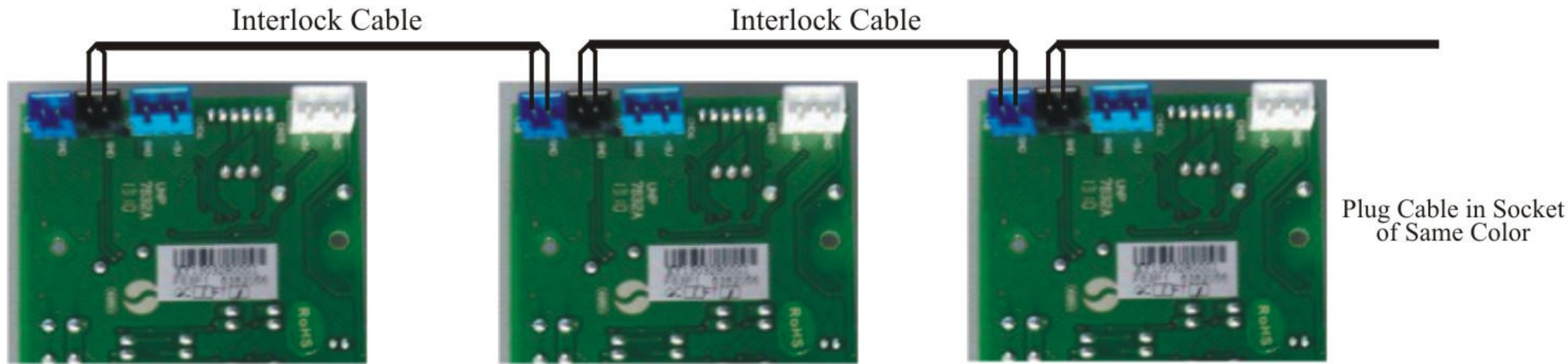
Figure 3-9 Network System Wiring with Interlock Cable
