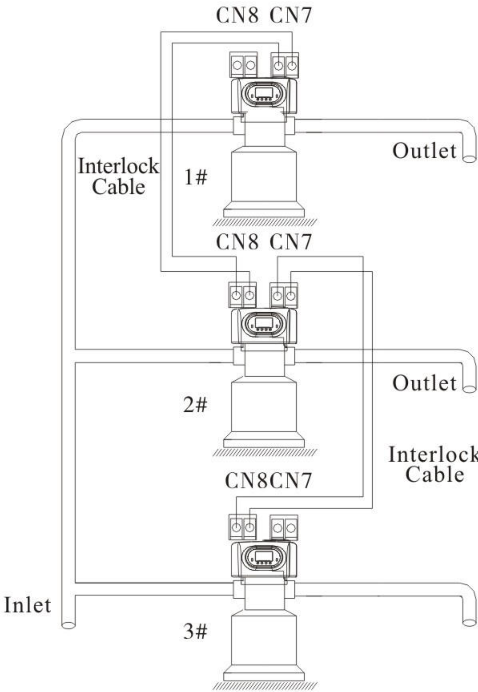
Figure 3-12 Interlock system
