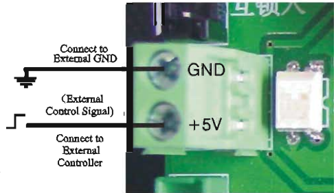
Figure 3-10 Wiring of Remote Input
