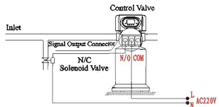
Figure 3-4 Wiring of Pressure Relief Connector
